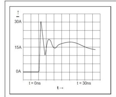
ESD Test Waveform for IEC61000-4-2
