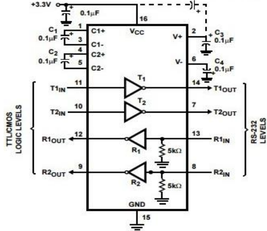
KY3232 C 3 (OPTIONAL CONNECTION,NOTE)
